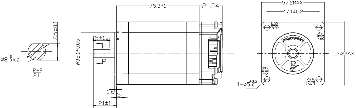
iCL57A-RS23
